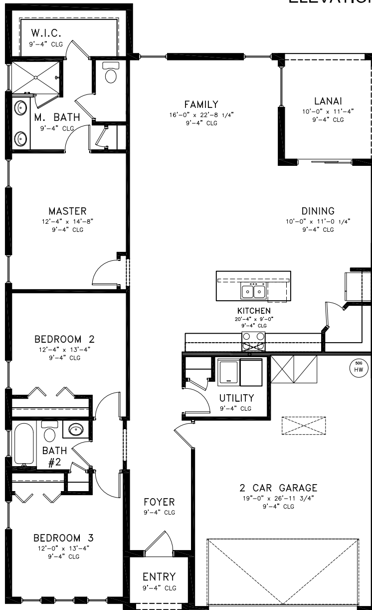
FLOOR PLAN
